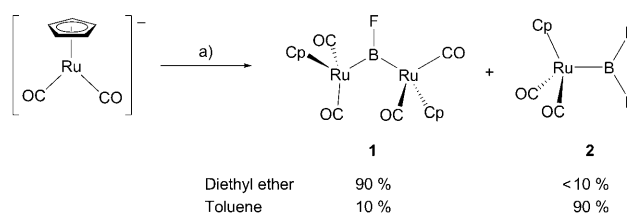
Scheme 2. Solvent-induced selectivity in the synthesis of fluoroborylene and difluoroboryl complexes 1 and 2 . Key reagents and conditions: a) BF 3 ·OEt 2 (0.58 equiv), diethyl ether, –78 to 20 °C, then a further 24 h at 20 °C, 90% conversion to 1 as determined by 11 B NMR spectroscopy (32% yield of isolated product). The analogous reaction in toluene under otherwise identical conditions leads to 90% conversion to 2 .
