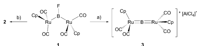
Scheme 4. Reactivity of fluoroborylene complex 1 : heterolytic cleavage of the BF bond by reaction with the Lewis acid \text{AlCl}_3 and thermolysis to give difluoroboryl complex 2 . Key reagents and conditions: a) \text{AlCl}_3 (3.3 equiv), dichloromethane, 12 h, 20^\circ\text{C} , 50% yield of isolated product. The 1:1 reactions with \text{AlCl}_3 and \text{B}(\text{C}_6\text{F}_5)_3 also generate 3 , although less cleanly. b) Toluene, 80^\circ\text{C} , 14 days, quantitative yield as determined by ^{11}\text{B} NMR spectroscopy.
